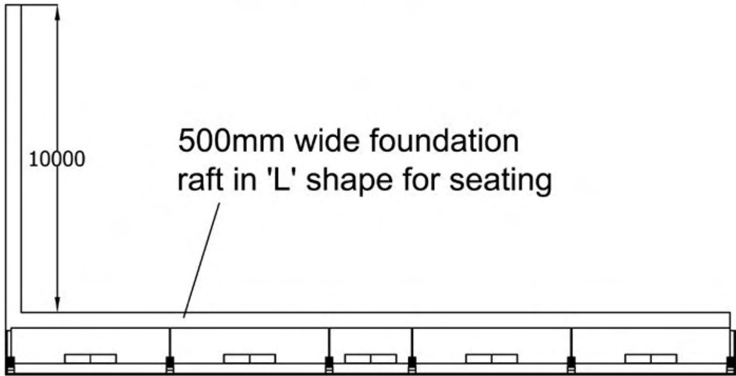
plan
